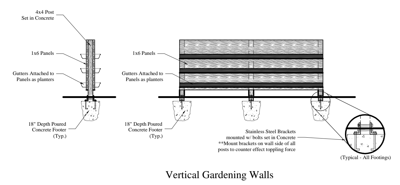
Vertical Gardening Walls Scale: 1/4" = 1'-0"
