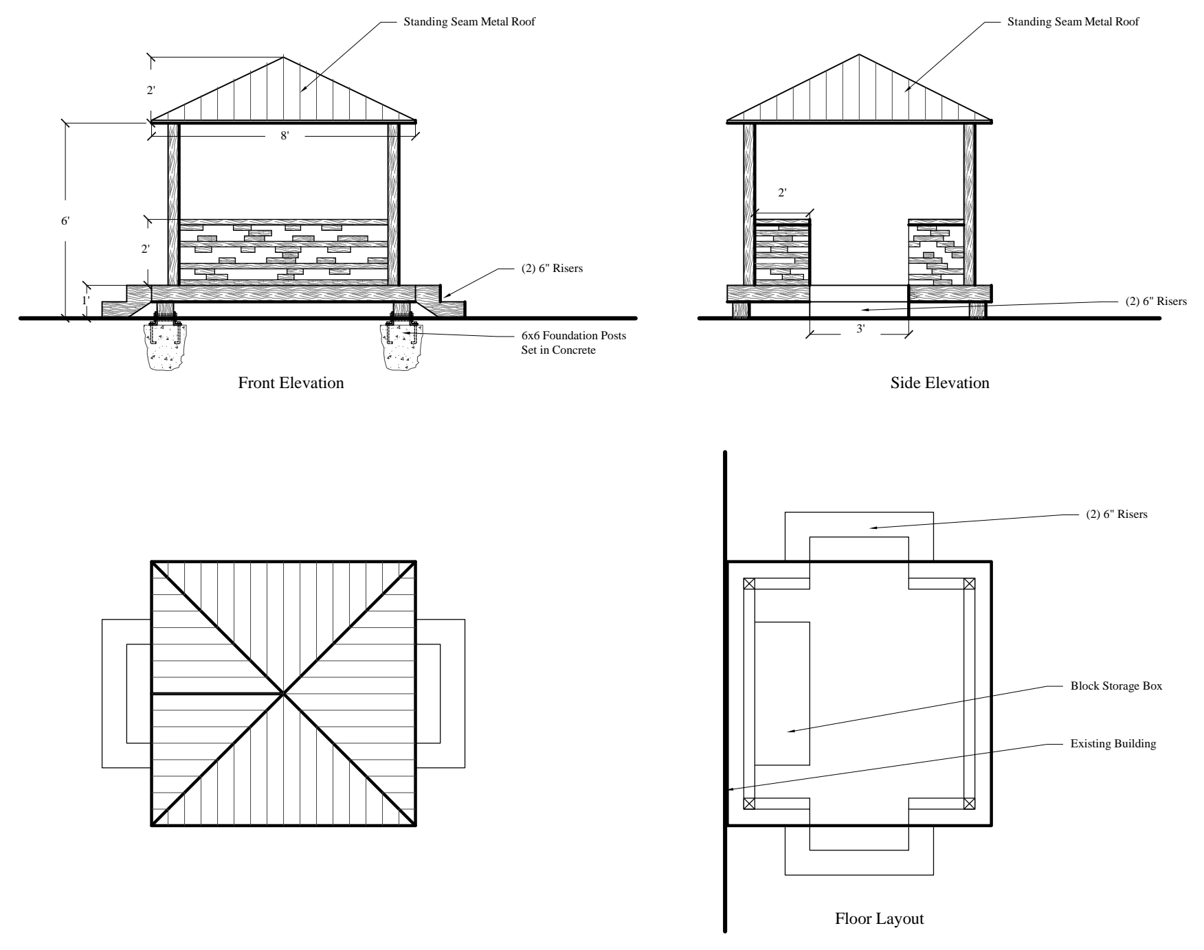
Building Block Platform Scale: 1/4" = 1'-0"
